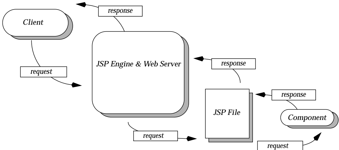
FIGURE 1-2 How Data is Passed Between the Client and the Server
